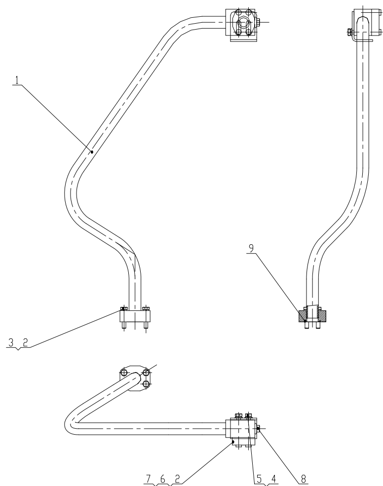
Z50G1011T16A 翻斗缸小腔硬管总成 Steel Tube Assembly
